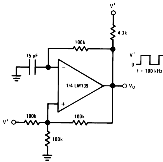
Squarewave Oscillator
