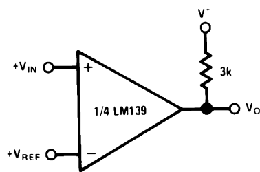
Basic Comparator
