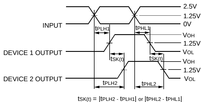
Part-to-Part Skew - t_{SK(PP)}
