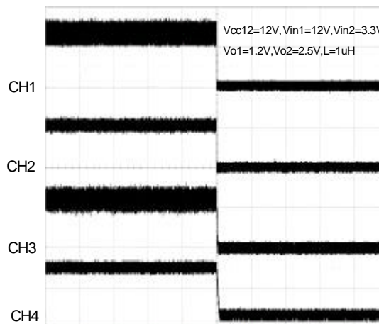
Shutdown(FS_DIS=GND)
