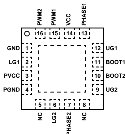
HIP6602BCR (16 LEAD QFN) TOP VIEW
